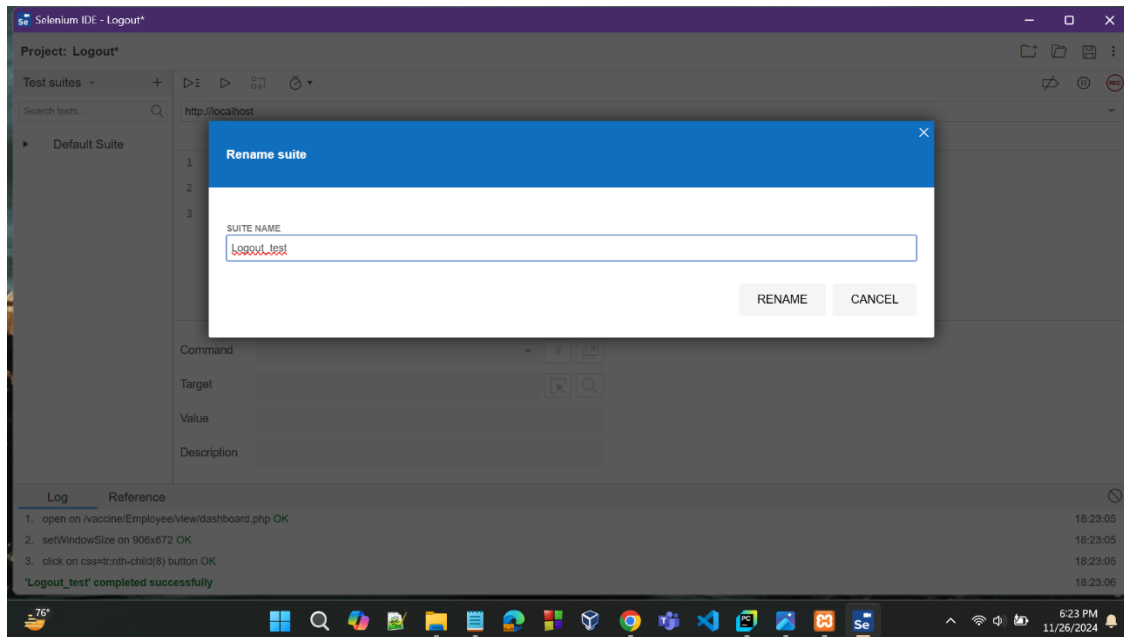
Fig 5: Suite Rename
