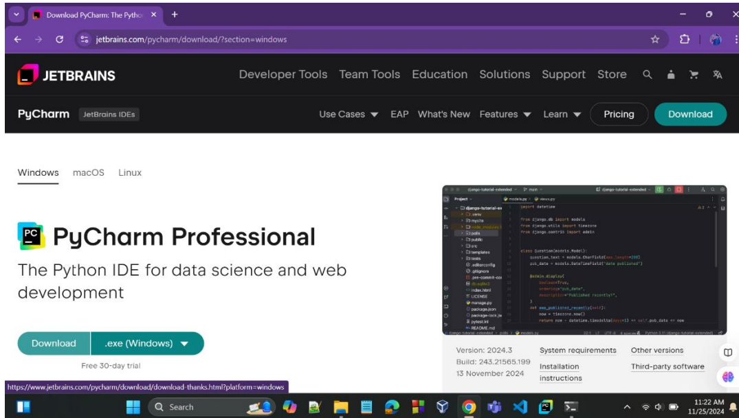
Fig 3: PyCharm Installation
