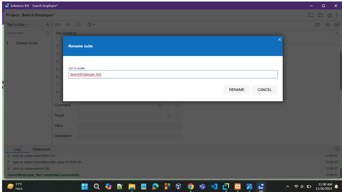
Fig 6: Rename Suite
