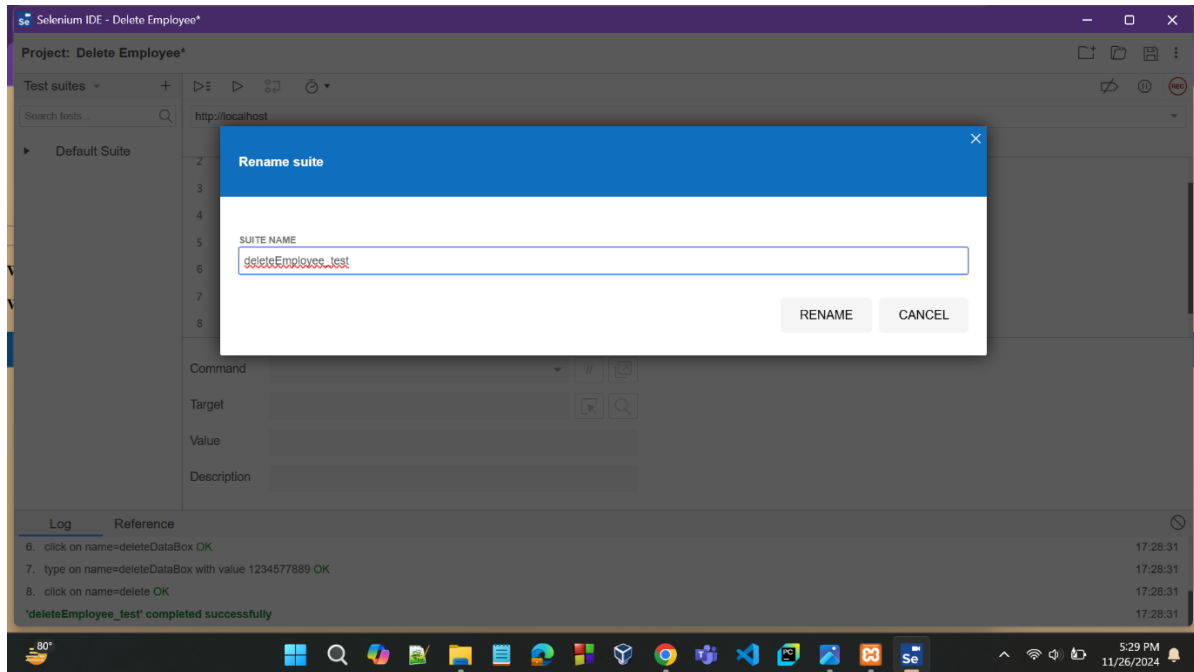
Fig 6: Rename Suite
