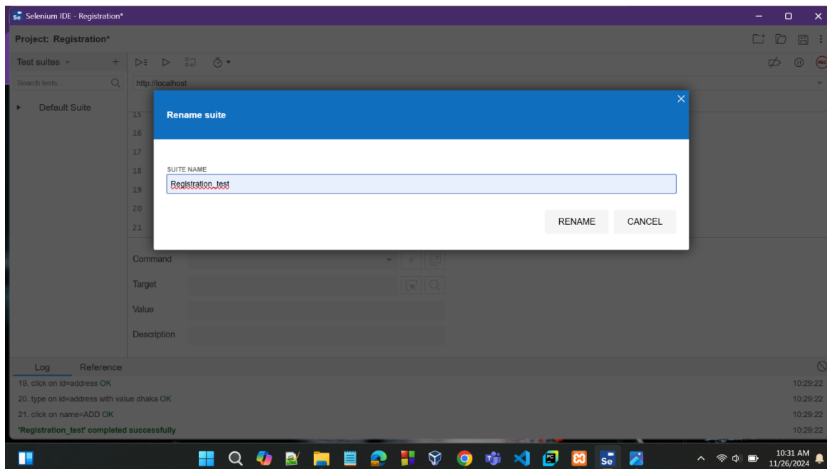
Fig 6: Rename Suite
