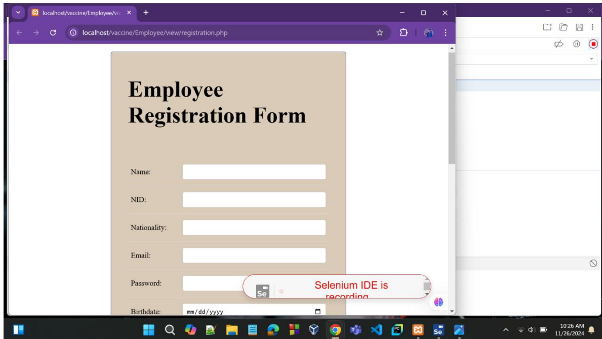
Fig 3: Complete Requirements
